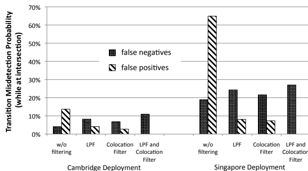
Figure 12: Transition filtering module evaluation. The transition filtering module removes false positive reports without significantly increasing the number of false negatives. The iPhone devices witnessed 219 and 37 traffic signal transitions in our Cambridge and Singapore deployments, respectively.
