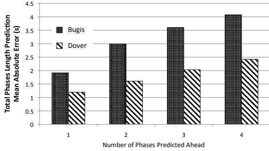
Figure 16: Evaluation of SignalGuru’s prediction scheme PS3 when predicting multiple phases ahead for Bugis and Dover traffic signals.
