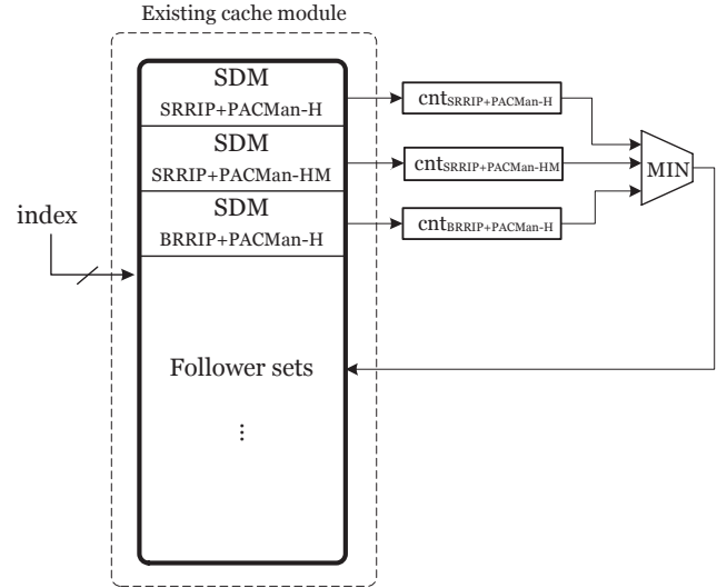
Figure 7: PACMan-DYN Implementation.
